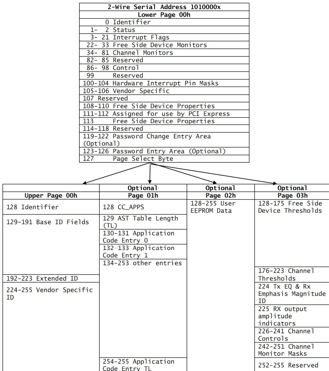
Figure 3, Memory Map
