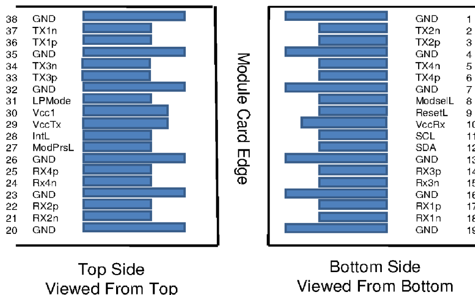
Figure 2, Pin View
